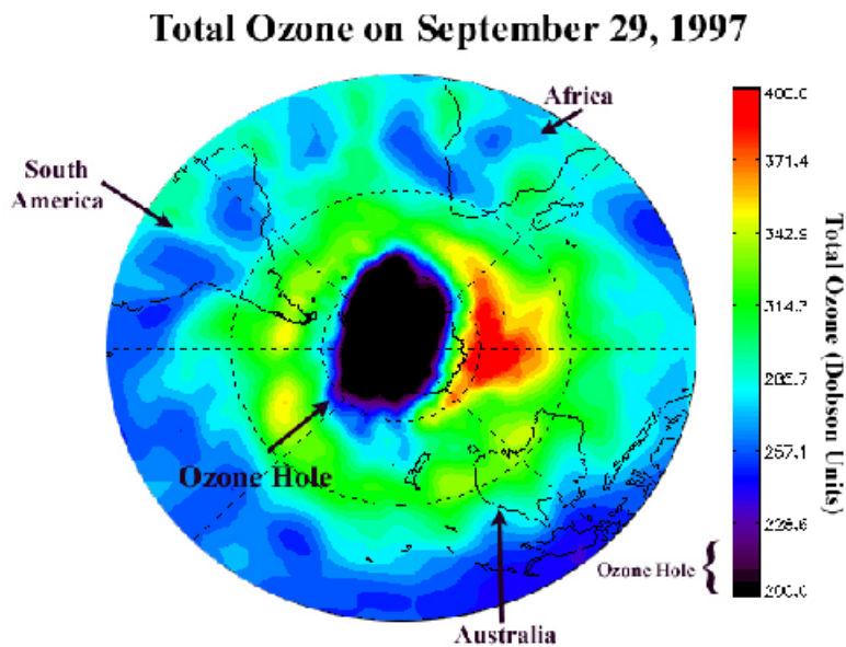
Figure 1. Southern Hemisphere view of total ozone on September 29, 1997 as calculated using the Monash University Transport Model. Large values of total ozone are indicated in the red, yellow and green colours, while the low values of ozone are indicated by purple and black. Note that the ozone hole is defined as a region where total ozone is below 220 Dobson units.
